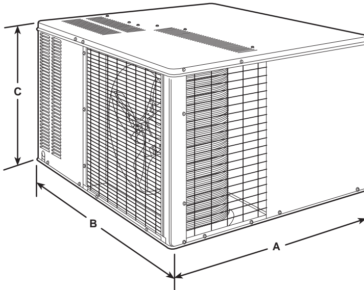
Base Unit Dimensions (Without Base Rail)
